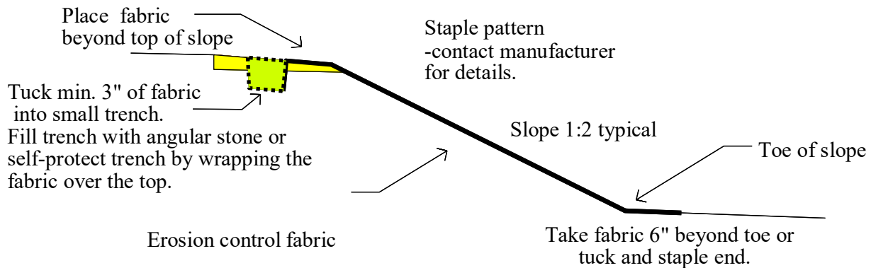
Figure 55 - Placement of an erosion fabric to protect a slope
