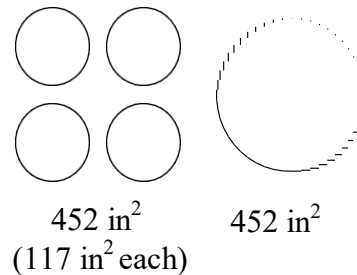
Figure 31 - 12" vs. 24" pipe
