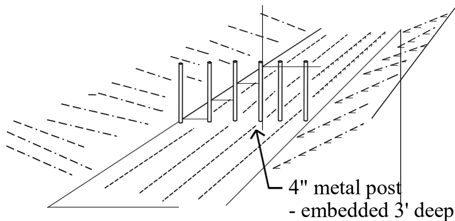
Figure 45 - Debris catcher
