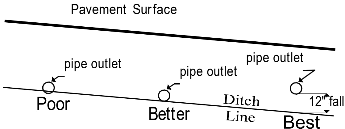
Figure 14 - Good and bad openings
