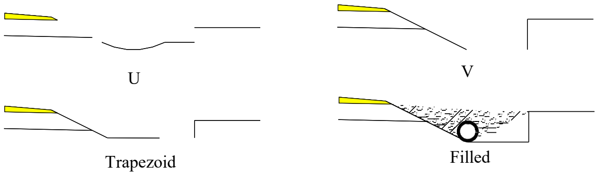
Figure 48 - Ditch shapes
