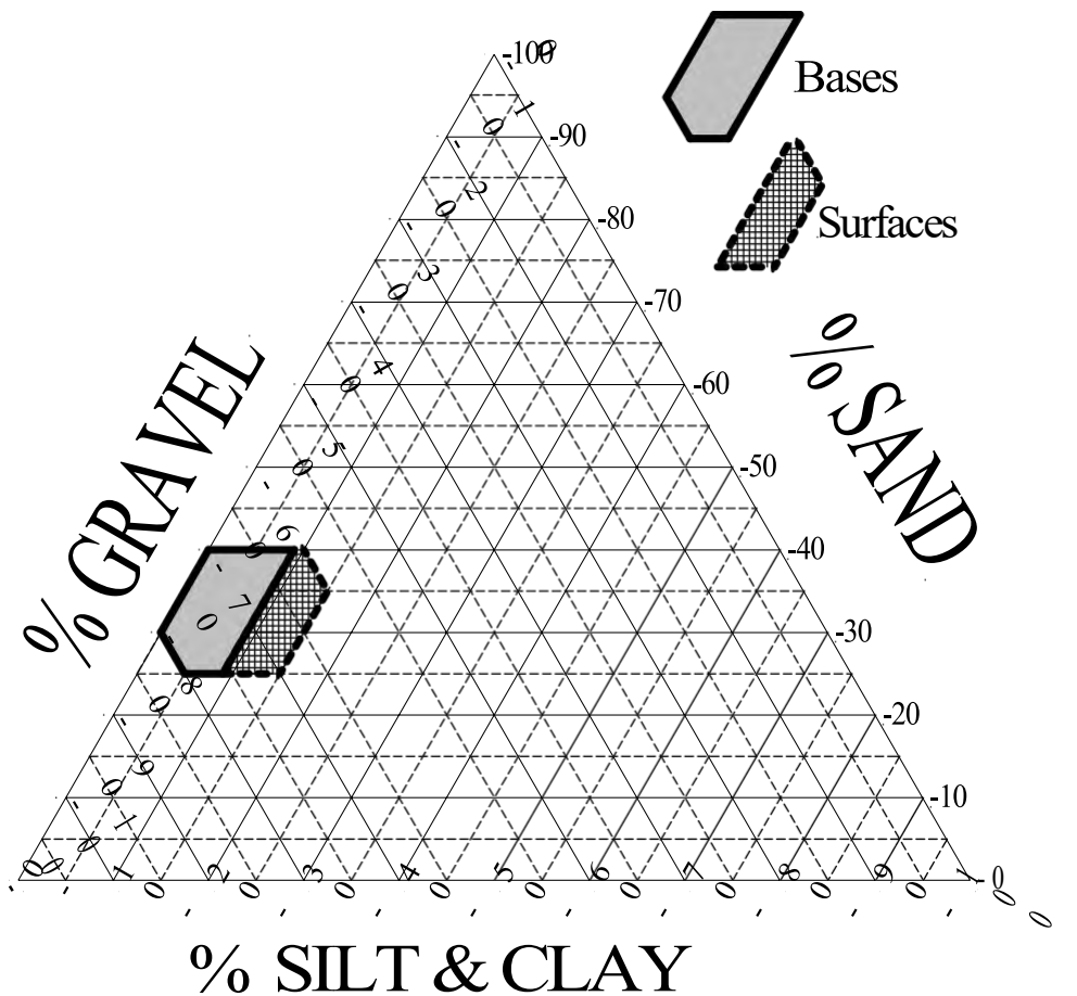
Figure 5 - Classification chart
